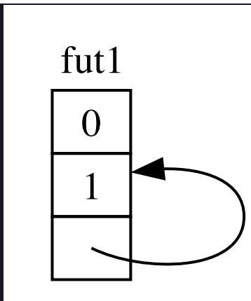
Figure 17-4: A self-referential data type.
