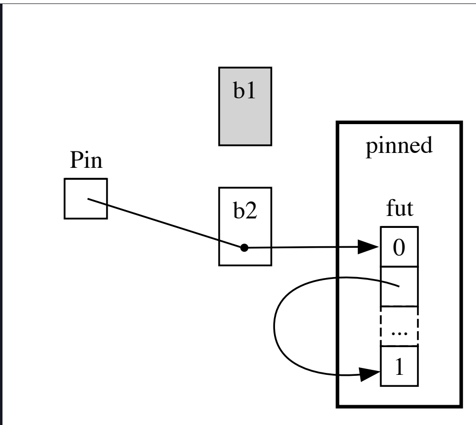
Figure 17-7: Moving a Box which points to a self-referential future type.
