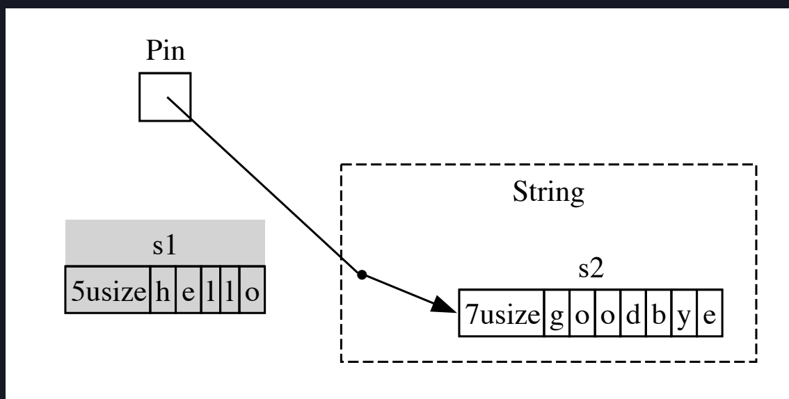
Figure 17-9: Replacing the String with an entirely different String in
