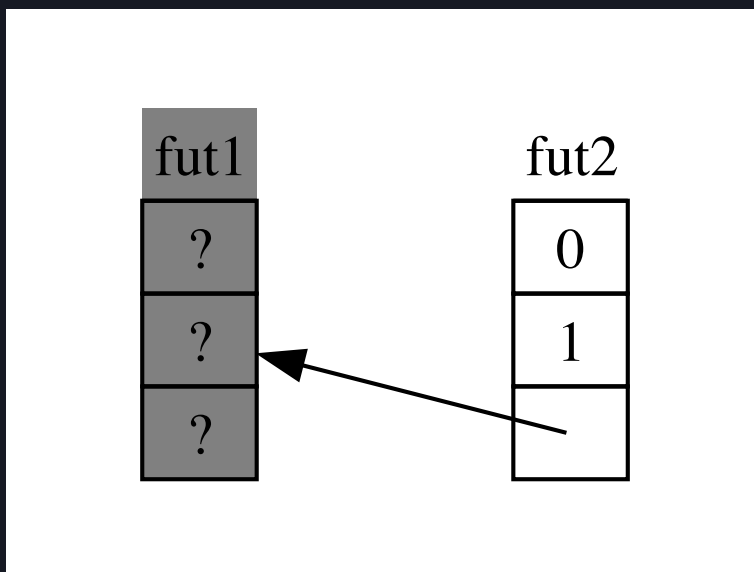
Figure 17-5: The unsafe result of moving a self-referential data type
