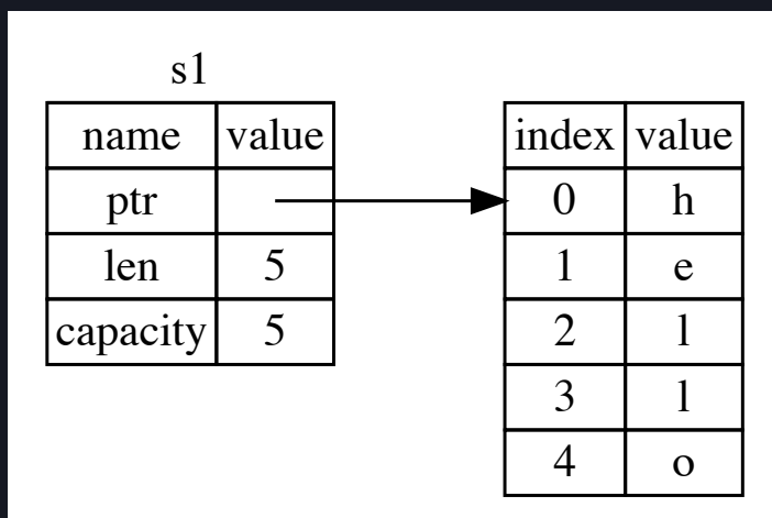
Figure 4-1: Representation in memory of a String holding the value "hello" bound to s1
